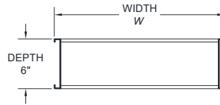
MODEL: 2620 FRAME: CHANNEL FRAME DUCT-MOUNT (DM)
