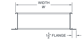
MODEL: 2625 FRAME: FLANGE FRAME FLANGE-MOUNT (FM)
